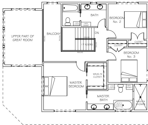
1122 SQ FT ON SECOND FLOOR
