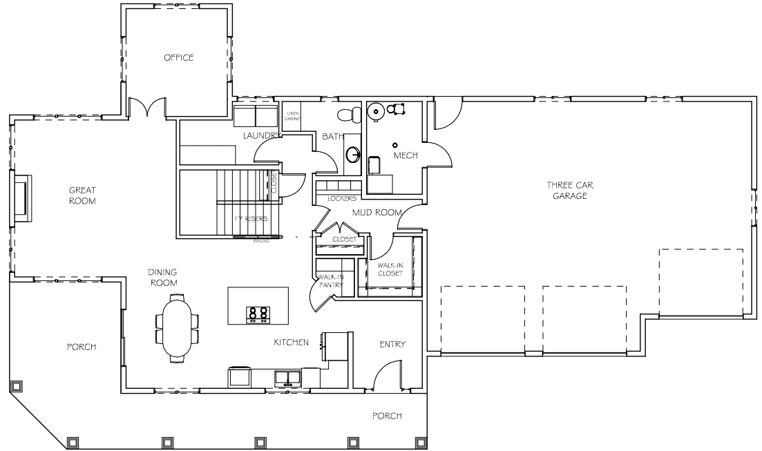
1334 SQ FT ON FIRST FLOOR
