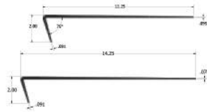
Hammered Tread (HMNT) 12 1/4" deep (HMNTD) 14" deep S M ▲ Z
